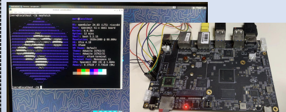
Banana Pi BPI-F3
